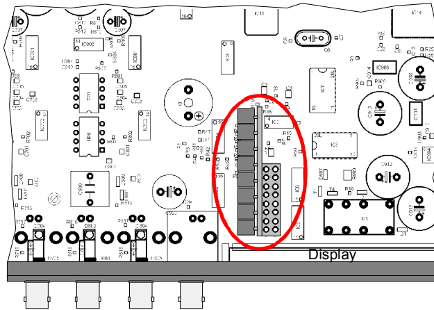
Figure 7: Location of the constant current source module
