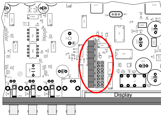
Figure 7: Location of the constant current source module
