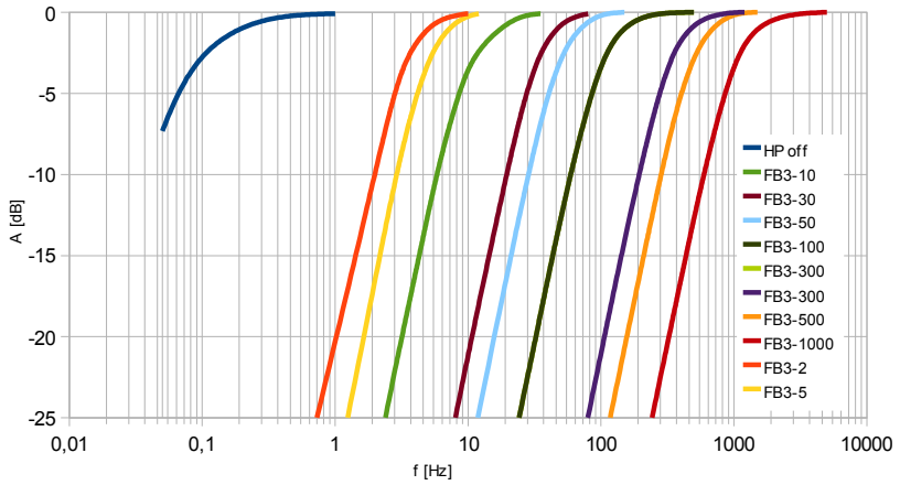
Figure 9: Frequency response of M208B with different high pass filters FB3-...
